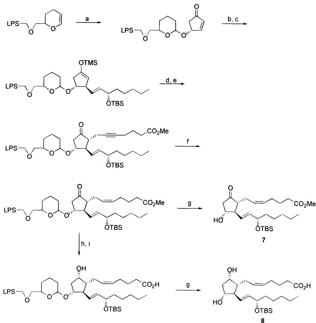
FIGURE 4. LPS-supported synthesis of prostaglandin E_2 methyl ester and prostaglandin F_{2\alpha} . Conditions: (a) 9 , PPTS, \text{CH}_2\text{Cl}_2 , room temperature, 24 h; (b) 10 , THF, -78^\circ\text{C} , 15 min; (c) (i) TMSCl, -78^\circ\text{C} , 30 min, (ii) \text{Et}_3\text{N} 0^\circ\text{C} , 15 min; (d) MeLi, THF -23^\circ\text{C} , 20 min; (e) 11 , -78^\circ\text{C} , 10 min then -23^\circ\text{C} , 30 min; (f) \text{H}_2 , 5% Pd– \text{BaSO}_4 , quinoline, benzene/cyclohexane (1:1), room temperature, 48 h; (g) 48% aqueous HF/THF (3:20, v/v), 45^\circ\text{C} , 6 h; (h) L-Selectride, THF, -78^\circ\text{C} , 1 h; (i) 3 N LiOH, THF, MeOH, room temperature, 48 h.
