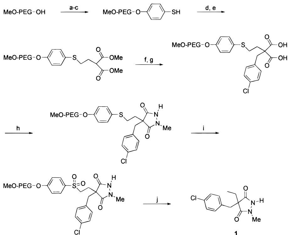
FIGURE 1. PEG-supported synthesis of 3,5-pyrazolidinediones. Conditions: (a) \text{MsCl} , \text{Et}_3\text{N} , \text{CH}_2\text{Cl}_2 , room temperature, 12 h; (b) 4\text{-HO-C}_6\text{H}_4\text{-S} , \text{Cs}_2\text{CO}_3 , DMF, 65^\circ\text{C} , 6 h; (c) DTT, \text{H}_2\text{O} , reflux, 3 h; (d) \text{BrCH}_2\text{CH}_2\text{Br} , \text{Cs}_2\text{CO}_3 , DMF, room temperature, 14 h; (e) \text{CH}_2(\text{CO}_2\text{Me})_2 , \text{Cs}_2\text{CO}_3 , DMF, room temperature, 17 h; (f) 4\text{-Cl-C}_6\text{H}_4\text{CH}_2\text{Cl} , \text{Cs}_2\text{CO}_3 , DMF, room temperature, 17 h; (g) (i) \text{NaOH} , \text{H}_2\text{O} , room temperature, 5 h, (ii) Amberlite IR-120 ( \text{H}^+ ), 1 h; (h) \text{CH}_3\text{NHNH}_2 , PyBOP, i\text{Pr}_2\text{EtN} , DMF, room temperature, 43 h; (i) \text{KHSO}_5 , \text{H}_2\text{O} , room temperature; (j) 5% \text{Na/Hg} , \text{Na}_2\text{HPO}_4 , \text{MeOH/DMF} (1/8), room temperature, 18 h.
